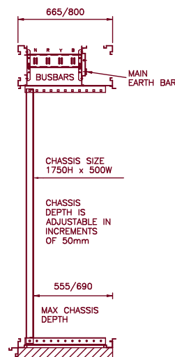
SECTION B-B
