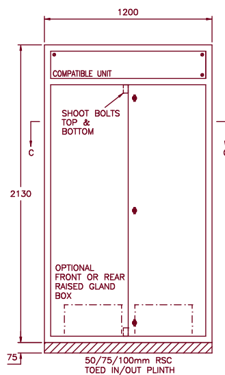
TYPICAL FRONT VIEW (DOUBLE DOOR TYPE)
