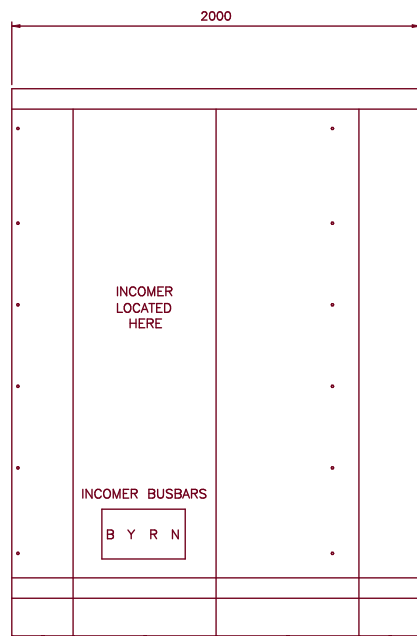
VIEW ON RH SIDE (INCOMER SIDE)
