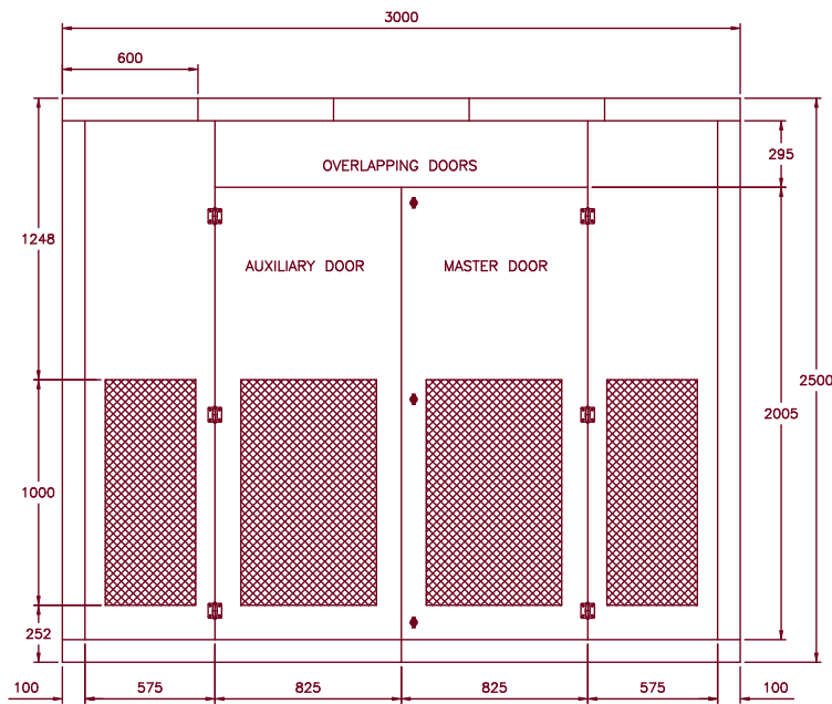
VIEW ON FRONT AND REAR
